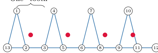
Comb Polygon with n = 13 vertices (requires 4 guards)
